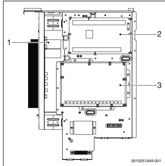
Afb. 63 Afmetingen CS2000AWF 18 R-T tot CS2000AWF 16 R-S/ CS2000AWF 30 R-T
