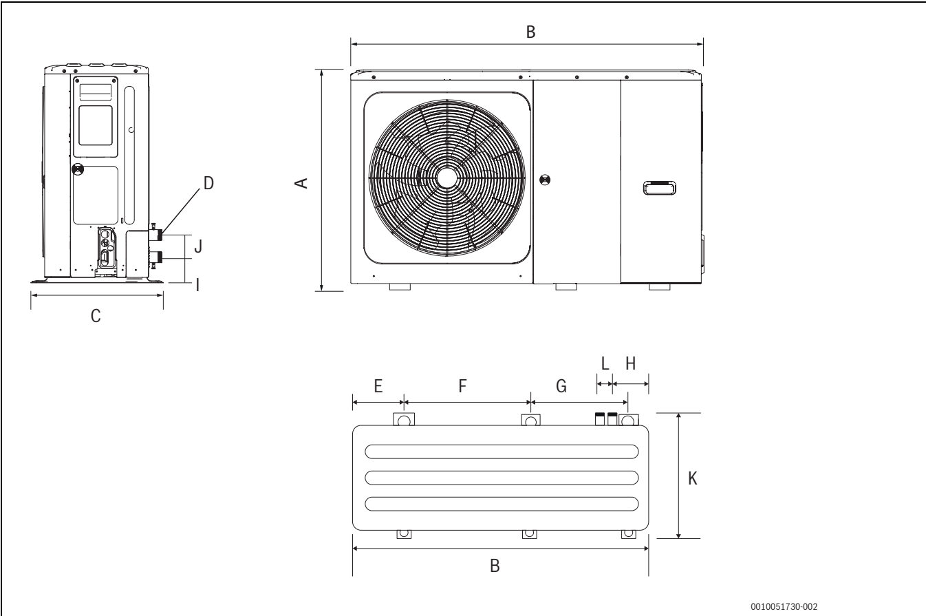
Afb. 33 Afmetingen CS2000AWF 8 R-S tot CS2000AWF 16 R-S/CS2000AWF 16 R-T
