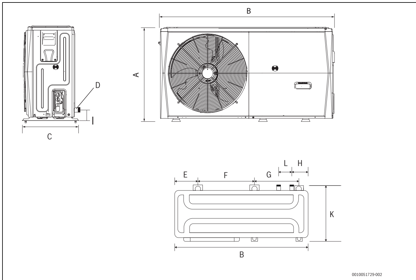
Afb. 32 Afmetingen CS2000AWF 4 R-S tot CS2000AWF 6 R-S
