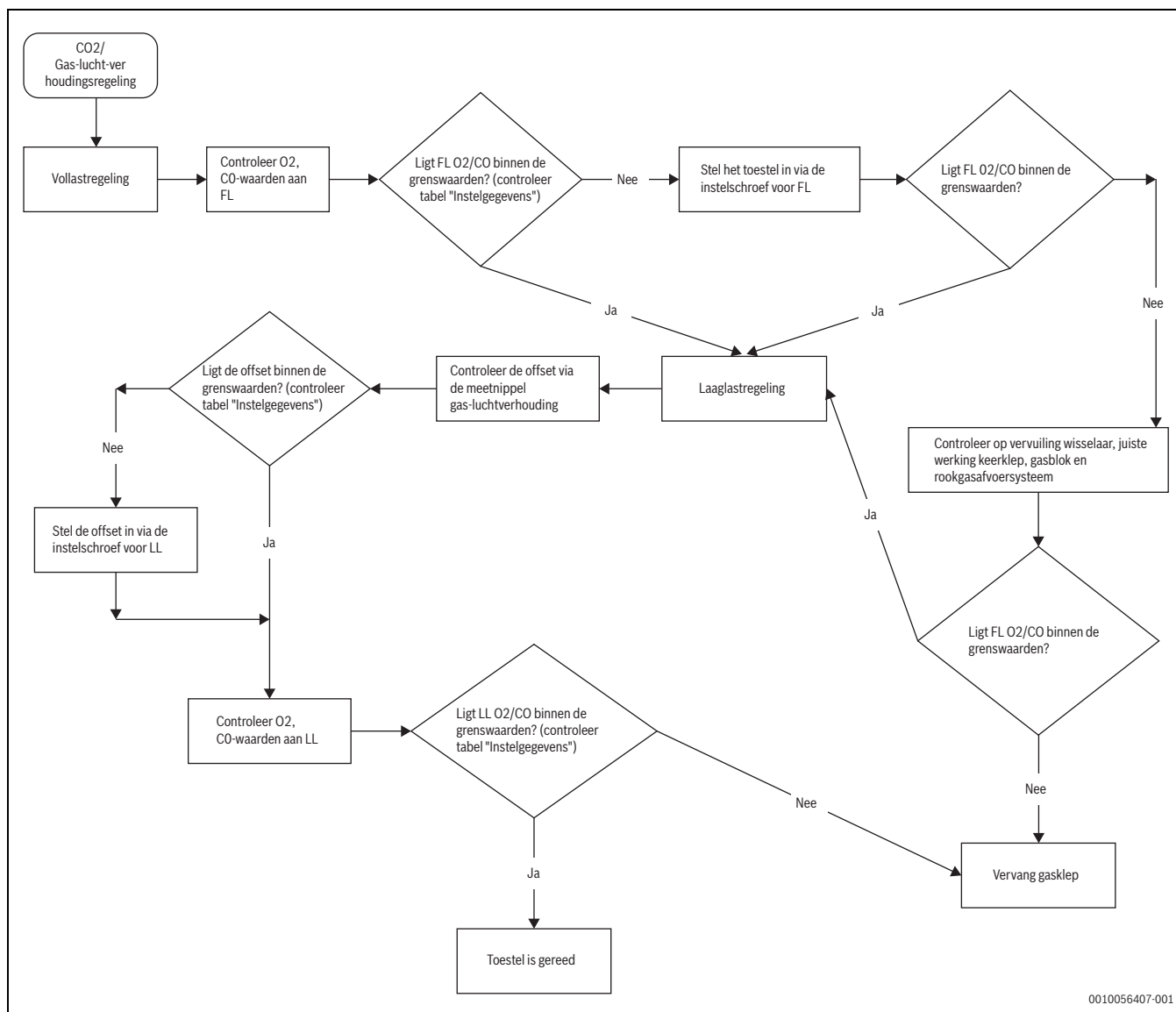
Afb. 34 Flowchart instelinstructions
